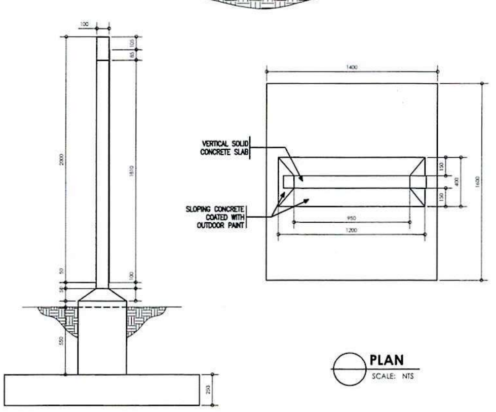
SITE MARKER FOUNDATION DETAILS SCALE: NTS
