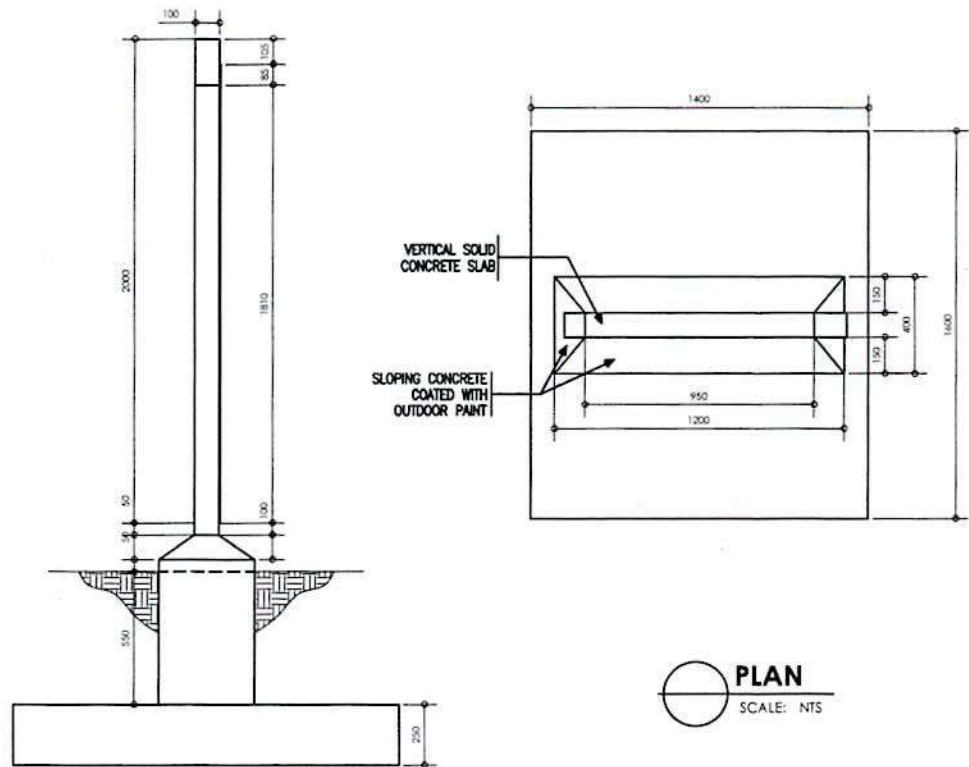
SITE MARKER FOUNDATION DETAILS SCALE: NTS
